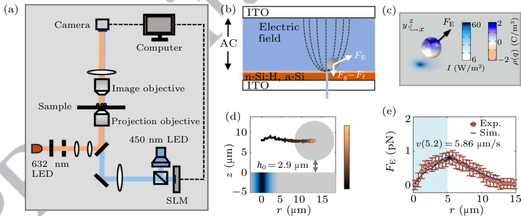
Fig. 1. Experimental setup and actuation mechanism. (a) Schematic of the feedback-controlled optoelectronic tweezer (OET) platform. (b) OET chip geometry and force components acting on a particle near a blue-light spot. The electrode gap H is 100 \mu\text{m} ; an AC voltage of 20 V_{pp} at 300 \text{ kHz} is applied. (c) Finite-element calculation of the induced charge density and the resulting dielectrophoretic (DEP) force near a circular blue-light spot. (d) Experimental three-dimensional particle trajectory measured by holographic microscopy; the equilibrium levitation height without blue light spot is h_0 = 2.9 \mu\text{m} . The blue shaded area indicates the projected light spot. (e) Variation of the mean radial DEP force F_E(r) with the lateral spot-particle distance. The blue line shows numerical results. The Gaussian blue-light spot has a full width at half maximum (FWHM) of 4.7 \mu\text{m} and a peak intensity of 6.06 \text{ mW/cm}^2 .
