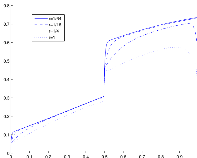
Fig. 5.2. Example 2. u_1(t) for r = 1, 1/4, 1/16, 1/64 .
