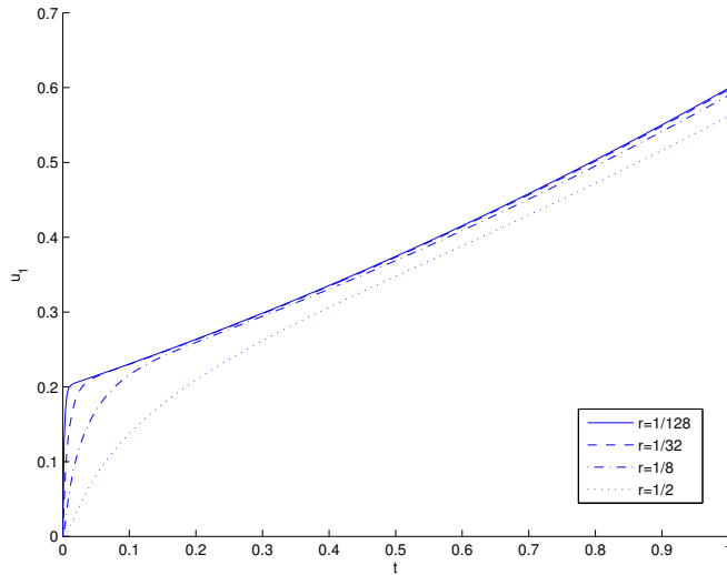
Fig. 5.1. Example 1. u_1(t) for r = 1/2, 1/8, 1/32, 1/128 .
