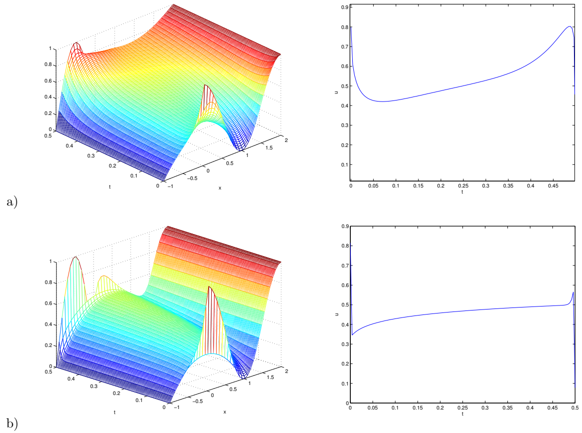
Fig. 5.3. Example 3. The numerical solution of the forward-backward parabolic problem. Left: u_i(t) for i = 1, 2, \dots, N ; Right: u_M where M satisfies x_M < 0 and x_{M+1} > 0 . a) p = 1 ; b) p = 10 . Here \Delta x = 1/40 , \Delta t = 1/256 .
