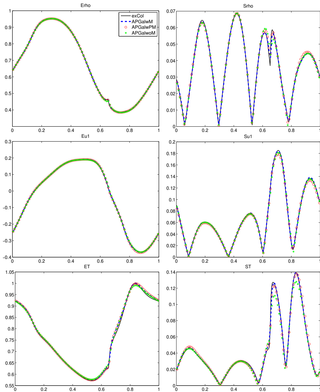
Figure 5: Mixed regime. Solutions at t = 0.1 . Left column: mean of \rho , u and T . Right column: standard deviation of \rho , u and T . Solid line: second-order explicit collocation with N_z = 20 , N_x = 200 , \Delta t = 2e - 5 . Dashed line: APGalwM. Circle: APGalwPM. Star: APGalwoM. For all three AP schemes K = 7 , N_x = 100 , \Delta t = 9.5e - 4 ( n_{\text{CFL}} = 0.8 ).
