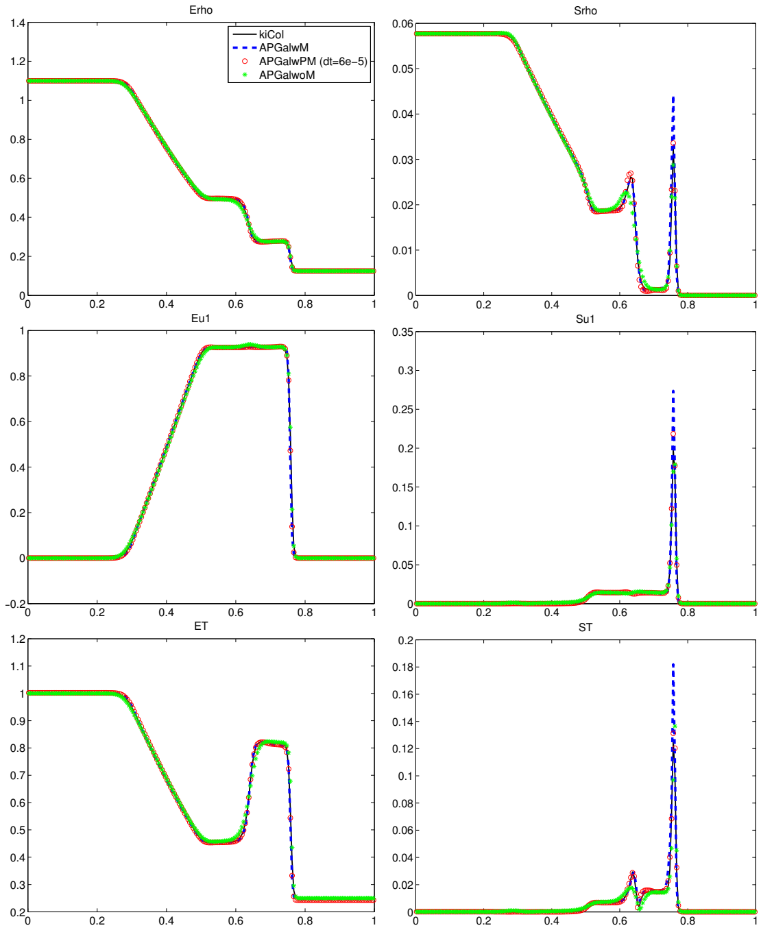
Figure 6: Shock tube problem. Case (I). \varepsilon = 1e - 6 . Solutions at t = 0.15 . Left column: mean of \rho , u and T . Right column: standard deviation of \rho , u and T . Solid line: second-order kinetic collocation with N_z = 20 , N_x = 200 , \Delta t = 4.8e - 4 ( n_{\text{CFL}} = 0.8 ). Dashed line: APGalwM. Circle: APGalwPM. Star: APGalwoM. For all three AP schemes K = 7 , N_x = 200 . \Delta t = 4.8e - 4 ( n_{\text{CFL}} = 0.8 ) for APGalwM and APGalwoM. \Delta t = 6e - 05 ( n_{\text{CFL}} = 0.1 ) for APGalwPM.
