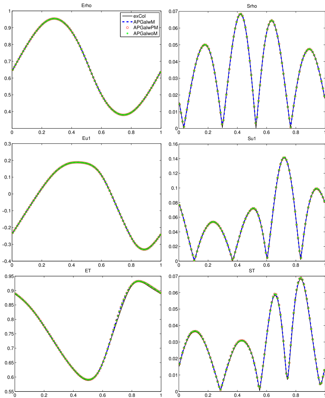
Figure 2: Kinetic regime \varepsilon = 1 . Solutions at t = 0.1 . Left column: mean of \rho , u and T . Right column: standard deviation of \rho , u and T . Solid line: second-order explicit collocation with N_z = 20 , N_x = 200 , \Delta t = 4.8e - 4 ( n_{\text{CFL}} = 0.8 ). Dashed line: APGalwM. Circle: APGalwPM. Star: APGalwoM. For all three AP schemes K = 7 , N_x = 100 , \Delta t = 9.5e - 4 ( n_{\text{CFL}} = 0.8 ).
