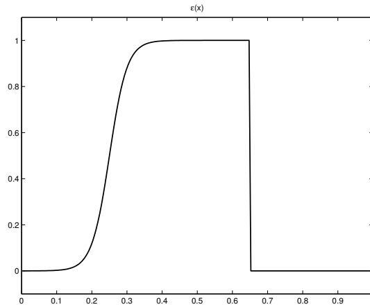
Figure 4: A spatially varying Knudsen number \varepsilon(x) .
