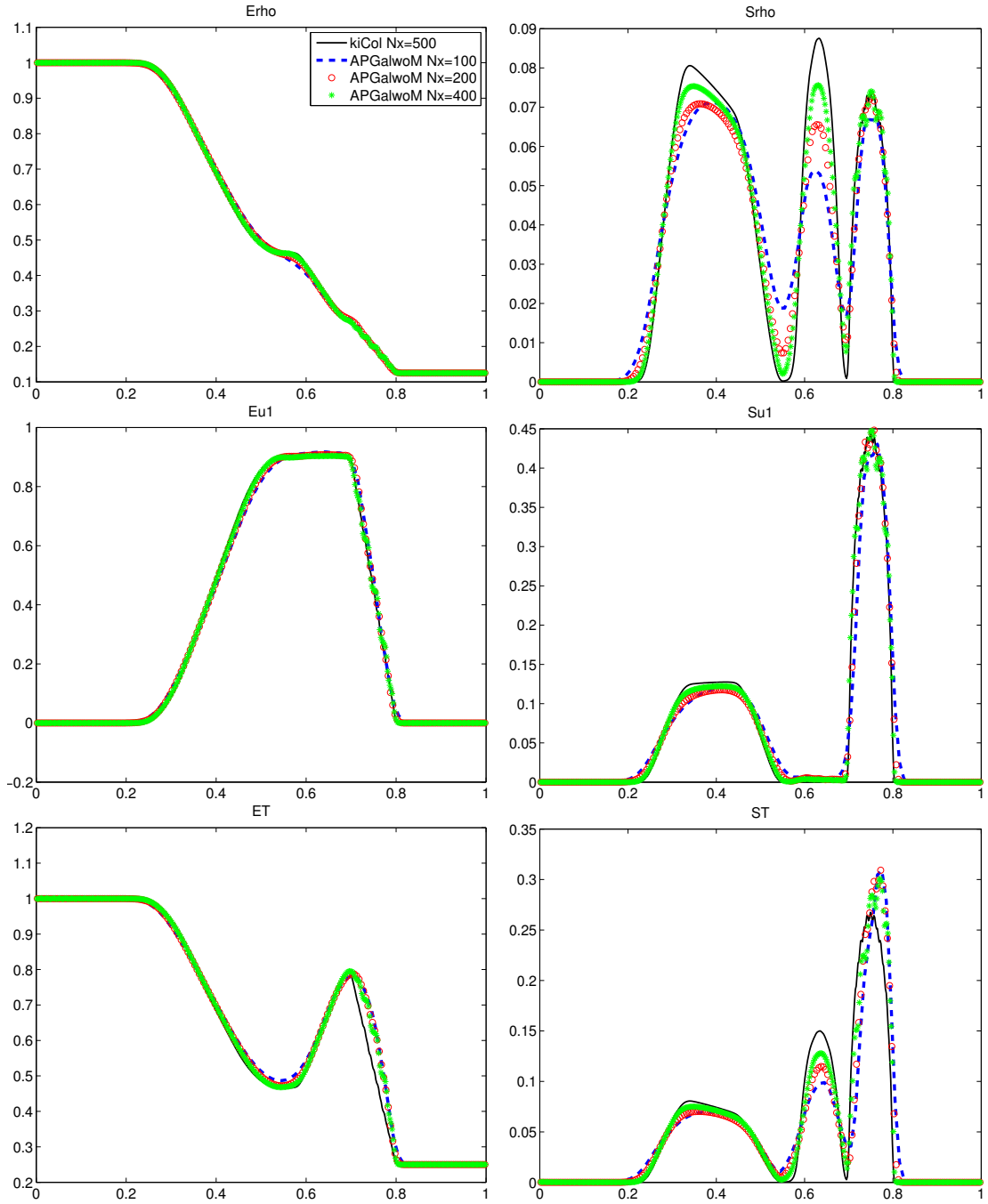
Figure 7: Shock tube problem. Case (II). \varepsilon = 1e - 6 . Solutions at t = 0.15 . Left column: mean of \rho , u and T . Right column: standard deviation of \rho , u and T . Solid line: second-order kinetic collocation with N_z = 20 , N_x = 500 , \Delta t = 1.9e - 4 ( n_{\text{CFL}} = 0.8 ). APGalwoM with K = 7 and various N_x (fixed n_{\text{CFL}} = 0.8 ).
