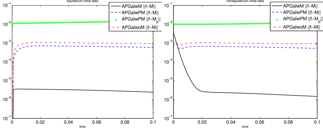
Figure 1: \|f - M\|_{L^2} versus time for different AP schemes. \varepsilon = 1e - 6 , K = 7 , N_x = 100 , \Delta t = 9.5e - 4 ( n_{\text{CFL}} = 0.8 ). Left: equilibrium initial data. Right: non-equilibrium initial data.
