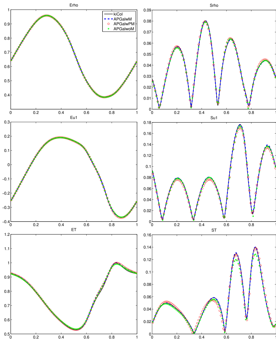
Figure 3: Fluid regime \varepsilon = 1e - 6 . Solutions at t = 0.1 . Left column: mean of \rho , u and T . Right column: standard deviation of \rho , u and T . Solid line: second-order kinetic collocation with N_z = 20 , N_x = 200 , \Delta t = 4.8e - 4 ( n_{\text{CFL}} = 0.8 ). Dashed line: APGalwM. Circle: APGalwPM. Star: APGalwoM. For all three AP schemes K = 7 , N_x = 100 , \Delta t = 9.5e - 4 ( n_{\text{CFL}} = 0.8 ).
