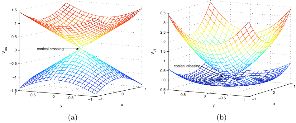
Figure 11.1. The conical crossings for potentials (a) V_{\text{iso}} and (b) V_{\text{JT}} defined in (11.3). The crossing point is (0, 0) for both potentials.
