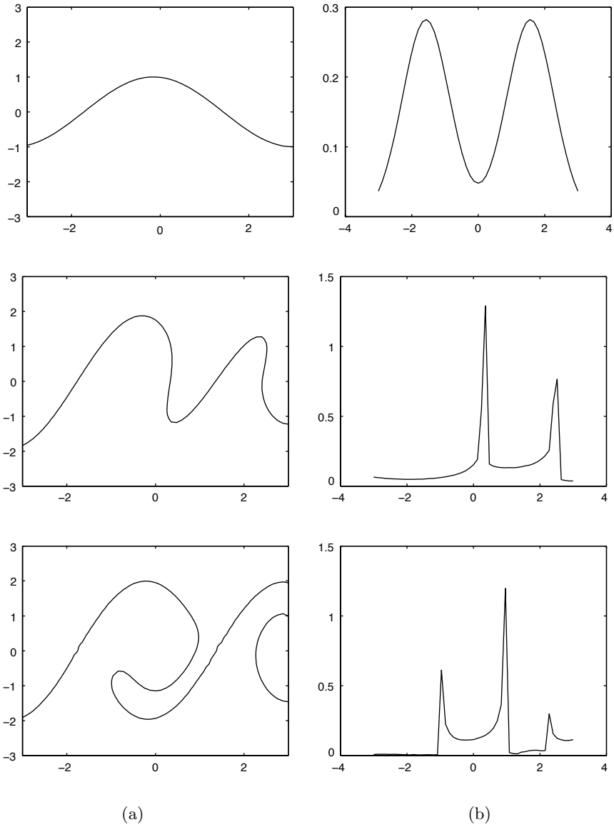
Figure 7.1. Example 7.1: (a) multivalued velocity v at time T = 0.0, 6.0, and 12.0 , (b) corresponding density \rho .
