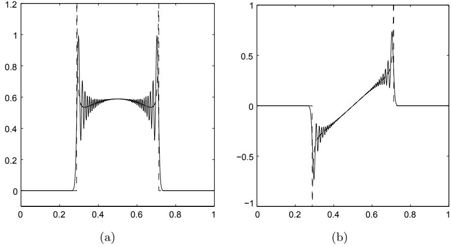
Figure 5.1. Numerical solution of (a) \rho^\varepsilon and (b) j^\varepsilon at t = 0.54 , as given in Example 5.5. In the figure, the solution computed by using SP2 for \varepsilon = 0.0008 , h = \frac{1}{512} , is superimposed, with the limiting \rho and j obtained by taking moments of the Wigner measure solution of (3.8).
