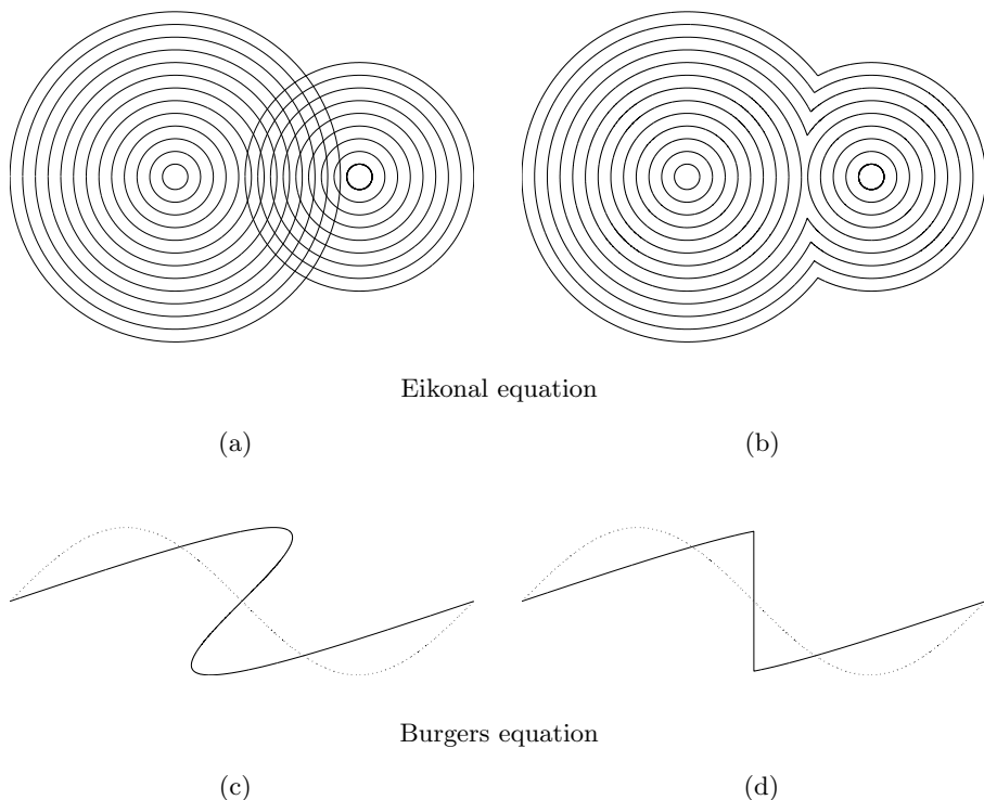
Figure 6.1. Multivalued solution ( left ) versus viscosity solution ( right ). (a, b) Zero-level set curves (at different times) of solutions to the eikonal equation (6.2). (c, d) Two solutions to the Burgers equation (6.3) before and after the formation of a shock.
