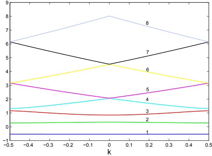
Figure 12.1. The eigenvalues E_m(k) , m = 1, \dots, 8 for Mathieu's model: V_\Gamma = \cos y .
