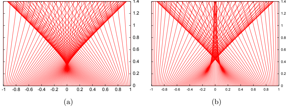
Figure 2.1. Caustics generated from initial data \partial_x S_{\text{in}}(x) = -\sin(\pi x)|\sin(\pi x)|^{p-1} : (a) p = 1 , and the solution becomes triple-valued; (b) p = 2 , and we exhibit single-, triple- and quintuple-valued solutions.
