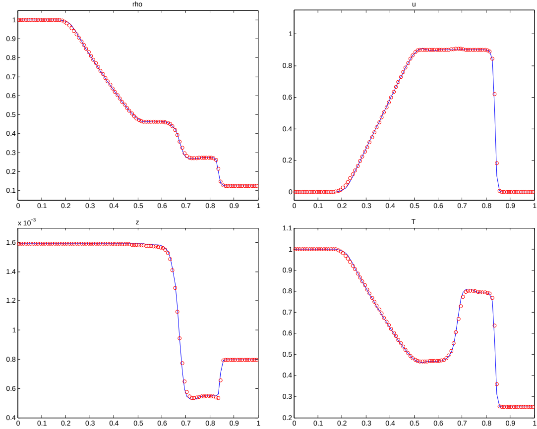
FIGURE 7. Bose gas. \epsilon = 1e - 4 , \theta_0 = 0.01 , z_l = 0.0016 , z_r = 7.9546e - 04 . Density \rho , velocity u , fugacity z , and temperature T at t = 0.2 . \Delta t = 0.0013 , \Delta x = 0.01 . Solid line: KFVS scheme [9] for quantum Euler equations (2.9); \circ : New scheme (4.4) for QBE (1.1).
