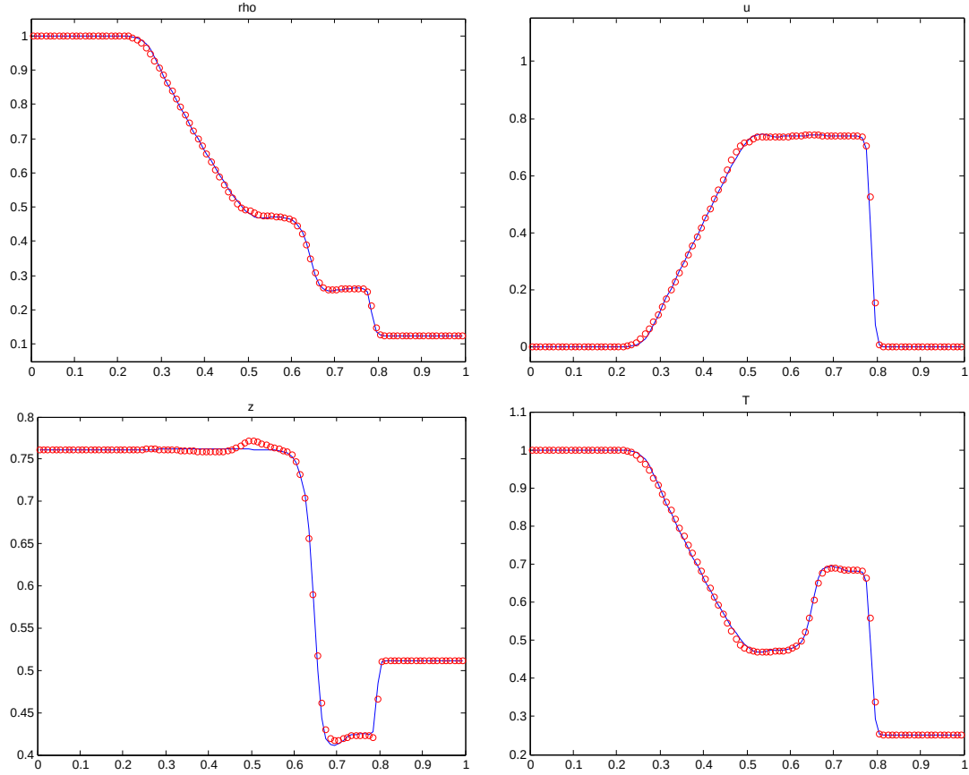
FIGURE 8. Bose gas. \epsilon = 1e-4 , \theta_0 = 9 , z_l = 0.7613 , z_r = 0.5114 . Density \rho , velocity u , fugacity z , and temperature T at t = 0.2 . \Delta t = 0.0017 , \Delta x = 0.01 . Solid line: KFVS scheme [9] for quantum Euler equations (2.9); \circ : New scheme (4.4) for QBE (1.1).
