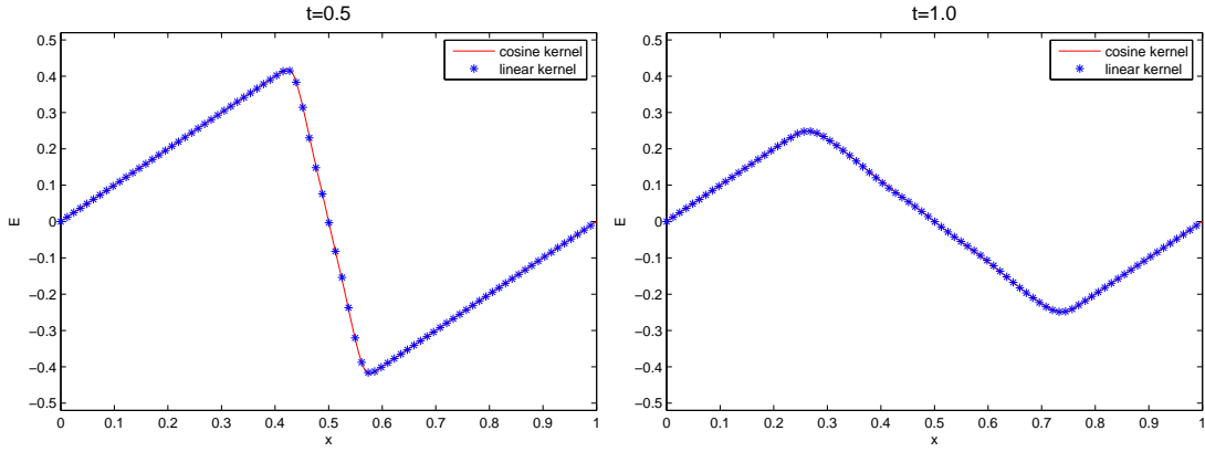
Figure 2: Example 4.1, comparison of the numerical solutions of the electric field E of the Schrödinger-Poisson equations with the cosine kernel approximation \delta_b^c in (4.1) and with the linear kernel approximation \delta_b^l in (4.2). The re-scaled Planck constant is \epsilon = 5 \times 10^{-5} , the constant C = 1 , \Delta x = \frac{1}{8192} and \Delta t = 0.005 .
