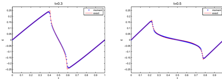
(c) Electric field
