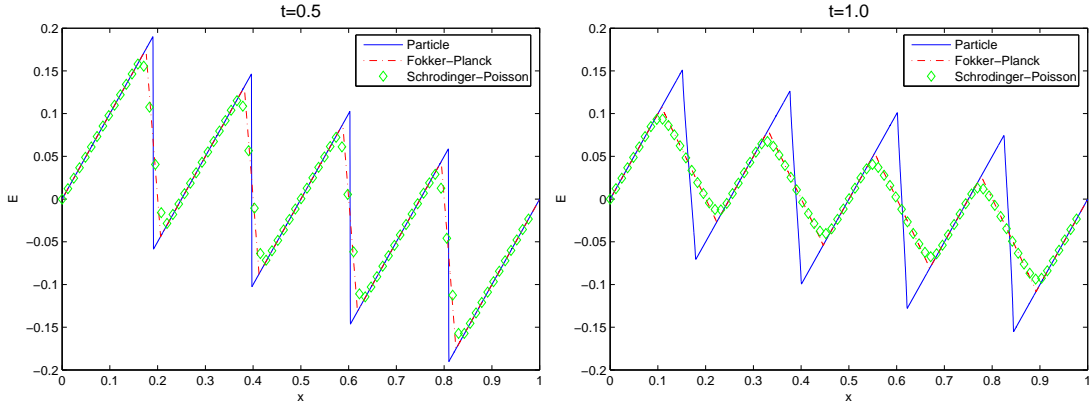
Figure 4: Example 4.2, four particles fission process. Comparison of the numerical solutions of the electric field E by the Vlasov-Poisson equations and the Fokker-Planck equations, both using the particle method, and the Schrödinger-Poisson equations. The parameters and mesh grids are the same as Figure 1 in Example 4.1. In the figures, “particle” solution refers to the solution of the Vlasov-Poisson equation by the particle method.
