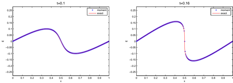
(c) Electric field
