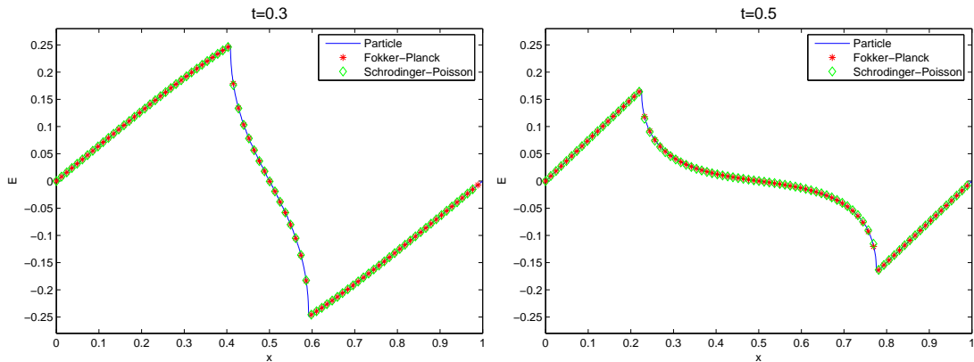
Figure 6: Example 4.4, comparison of the numerical solutions of the electric field E by the Vlasov-Poisson equations and the Fokker-Planck equations, both using the particle method, and by the Schrödinger-Poisson equations. Particle number N = N^* = 8192 , kernel mollifier parameter \delta = 0.001 , \Delta t = 0.002 . The viscosity for the Fokker-Planck equation is \eta = 0.001 . In the Schrödinger-Poisson, the re-scaled Planck constant is \epsilon = 5 \times 10^{-5} , the constant C = 1 , \Delta x = \frac{1}{8192} and \Delta t = 0.005 .
