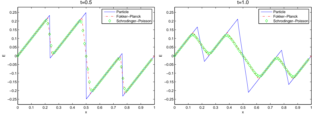
Figure 3: Example 4.2, three particles fission process. Comparison of the numerical solutions of the electric field E by the Vlasov-Poisson equations and the Fokker-Planck equations, both using the particle method, and the Schrödinger-Poisson equations. The parameters and mesh grids are the same as Figure 1 in Example 4.1. In the figures, “particle” solution refers to the solution of the Vlasov-Poisson equation by the particle method.
