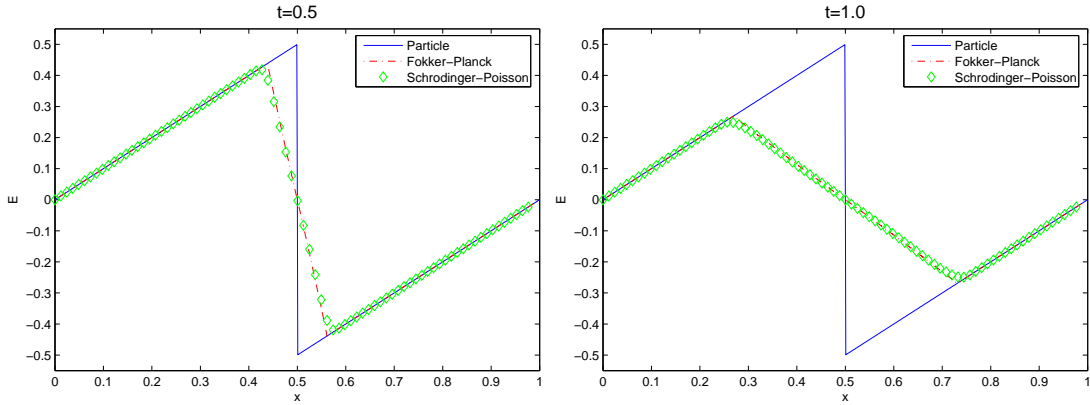
Figure 1: Example 4.1, comparison of the numerical solutions of the electric field E by the Vlasov-Poisson equations and the Fokker-Planck equations, both using the particle method, and the Schrödinger-Poisson equations. Particle number N = N^* = 8192 , kernel mollifier parameter \delta = 0.001 , \Delta t = 0.002 . The viscosity coefficient for the Fokker-Planck equations is \eta = 0.001 . In the Schrödinger-Poisson equations, we use the re-scaled Planck constant \epsilon = 5 \times 10^{-5} , the constant C = 1 , \Delta x = \frac{1}{8192} , \Delta t = 0.005 and \delta_b^\epsilon given in (4.1). In the figures, “particle” solution refers to the solution of the Vlasov-Poisson equation by the particle method.
