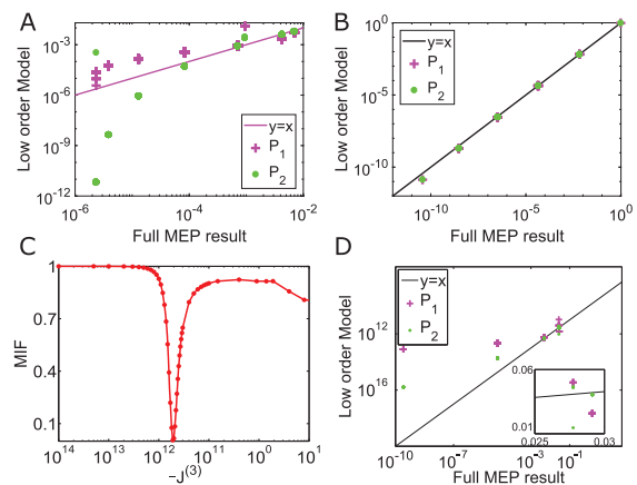
Fig. 1: MEP analysis using numerically constructed probability distribution. As in the text, J^{(1)} , J^{(2)} , J^{(3)} , J^{(4)} are the first-, second-, third- and fourth-order effective interaction strength, respectively. For (a), (b) and (d), the MEP probability P_2 (green), and P_1 (magenta) of firing states is shown against the full MEP distribution P_n . Each data point here corresponds to a particular network state. The case in (a) has the MIF of 92% for 10 nodes. J^{(1)} = 0 , J^{(2)} = 0 , J^{(3)} = 0.5 , J^{(4)} = -0.2857 , J^{(k)} \equiv 0 for 5 \leq k \leq 10 . Points with probability smaller than 10^{-20} are not plotted. The case in (b) has the MIF of 12% for 5 nodes. J^{(1)} = -5 , J^{(2)} = 0.001 , J^{(3)} = 0.1 , J^{(k)} \equiv 0 for 4 \leq k \leq 5 . The constructed MEP probabilities P_1 and P_2 using these J 's overlap each other rather well. (c) MIF vs. the third-order effective interaction. Here we use 7 nodes, J^{(1)} = 0 , J^{(2)} = 0.05 , J^{(k)} \equiv 0 for 4 \leq k \leq 7 . The case in (d) is one of cases in (c) for J^{(3)} = -1.9 . The MIF is 91.5%. Points with probability smaller than 10^{-10} are not plotted. The inset zooms in to a region of the comparison between the full MEP distribution P_n and P_2 .
